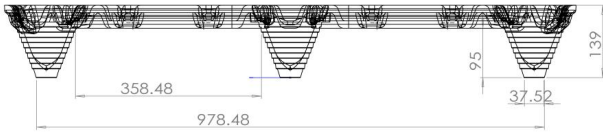
End View
